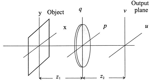
FIGURE 1. Single lens optical system.
