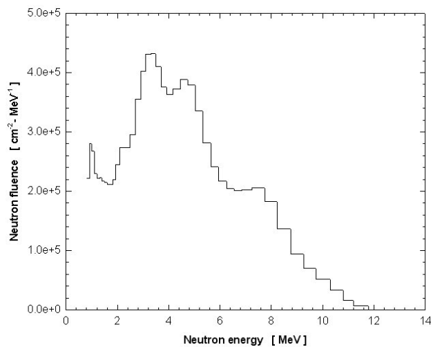
FIGURE 2. ^{239}\text{PuBe} neutron source spectrum.
