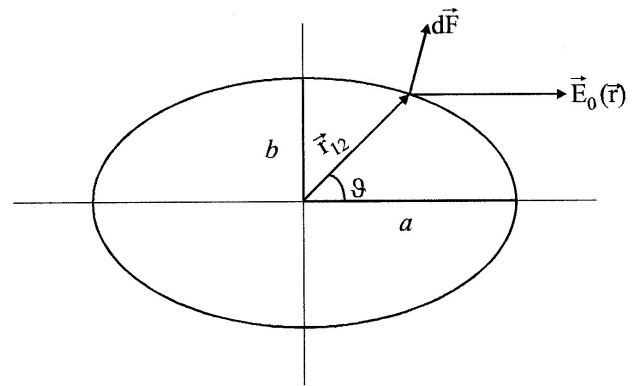
FIGURE 1. Prolate ellipsoid.
