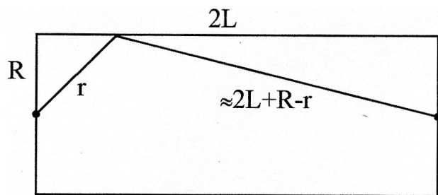
FIGURE 3. Long cylinder.
