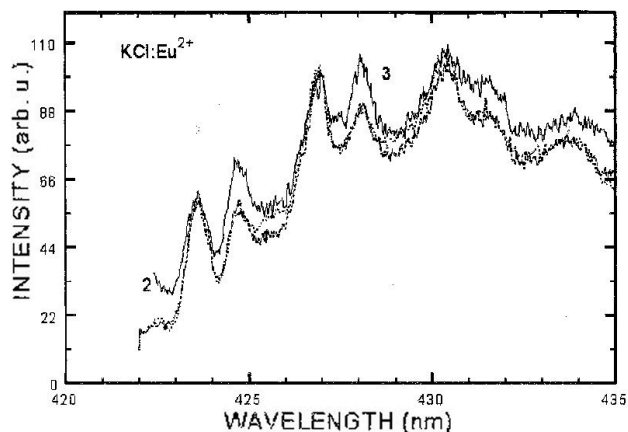
FIGURE 6. Emission spectra of a well-aged \text{KCl:Eu}^{2+} crystal for excitations at 418.6, 420 and 421 nm.
