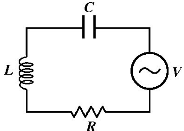
FIGURE 1. A typical representation of a RLC circuit.
