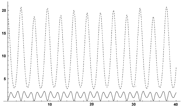
FIGURE 4a. Dispersion for Schrödinger cat state of \langle x^2 \rangle y \langle p^2 \rangle . Stable case. --- \langle x^2 \rangle , — \langle p^2 \rangle
