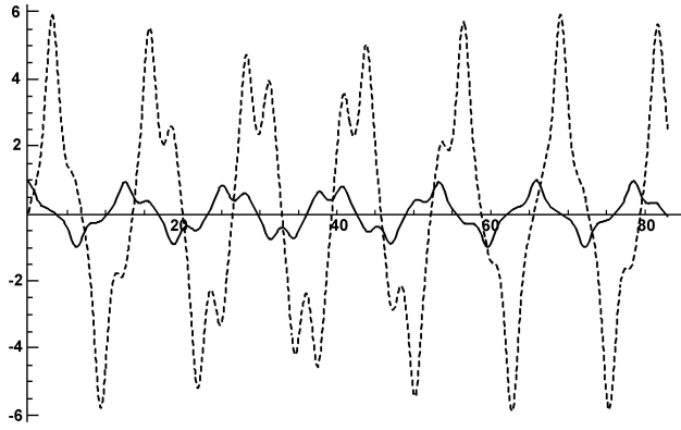
FIGURE 3a. Real and imaginary parts of the Mathieu function for the stable case: (a = -0.1, q = 0.75) --- Im(f), — Re(f)
