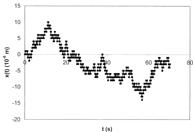
FIGURE 12A. Position of PM-2.5 (radius of 1.25 \times 10^{-6} m) particles as a function of time. The particles have an erratic motion whose amplitude seems to depend on the mass.
