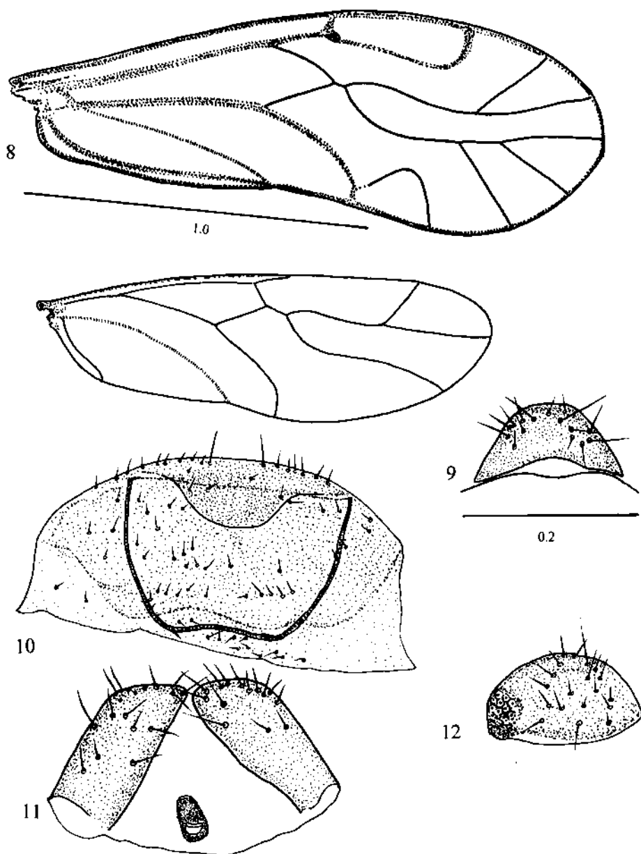
Figs. 8-12. Lachesilla mombachensis n. sp. (♀). 8. Fore- and hindwings. 9. Epiproct. 10. Subgenital plate. 11. Gonapophyses and ninth sternum. 12. Left paraproct. Scales in mm. Figs. 10-12 to scale of Fig. 9.
