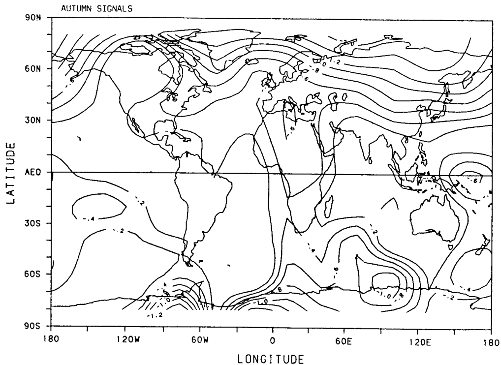
Fig. 7b. Similar to Fig. 5a, but autumn.
