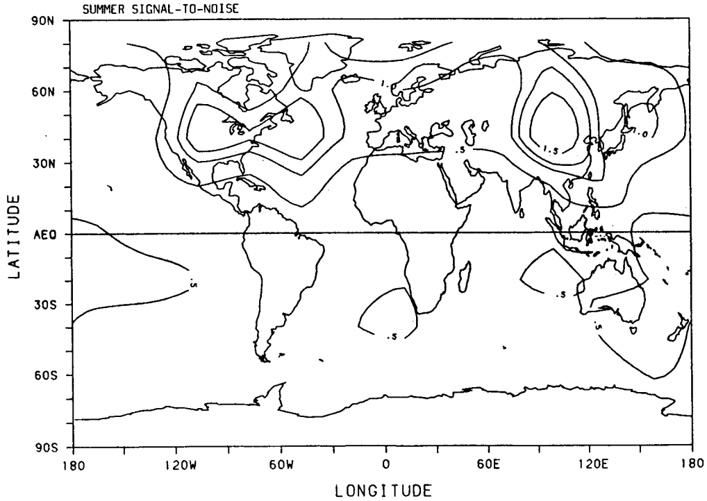
Fig. 6b. Similar to Fig. 6a, but summer.
