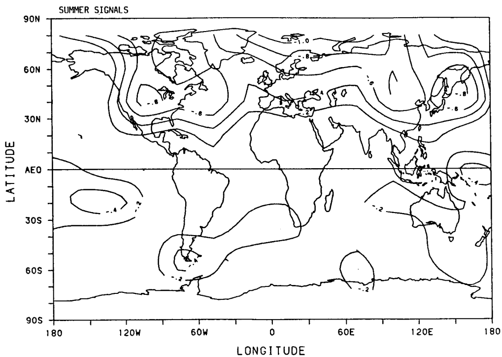
Fig. 5b. Similar to Fig. 5a, but summer.
