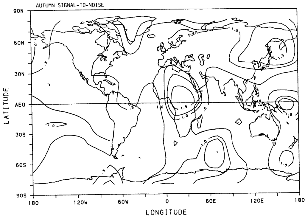
Fig. 8b. Similar to Fig. 8a, but autumn.
