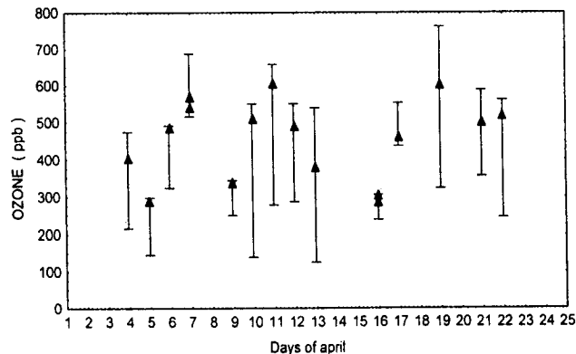
Fig. 4c. Variations in O_3 (max) in control bag conditions represented by triangles and perturbed chambers.
