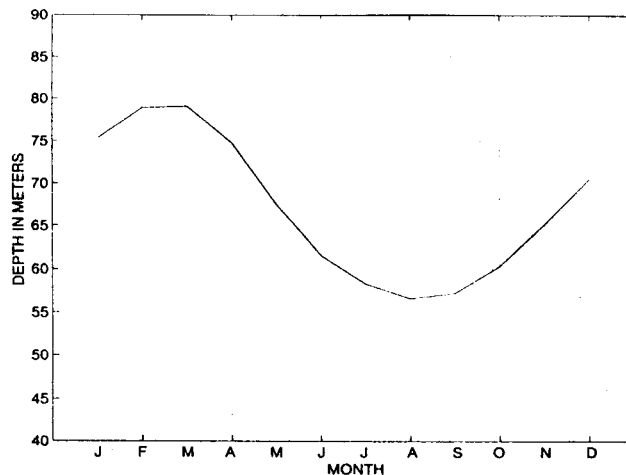
Fig. 11. Annual cycle of the mean upper layer thickness. It shows the seasonal variation of the mean upper layer thickness, maximum depth is reached in February and minimum in August. This cycle is determined by the entrainment and detrainment.
