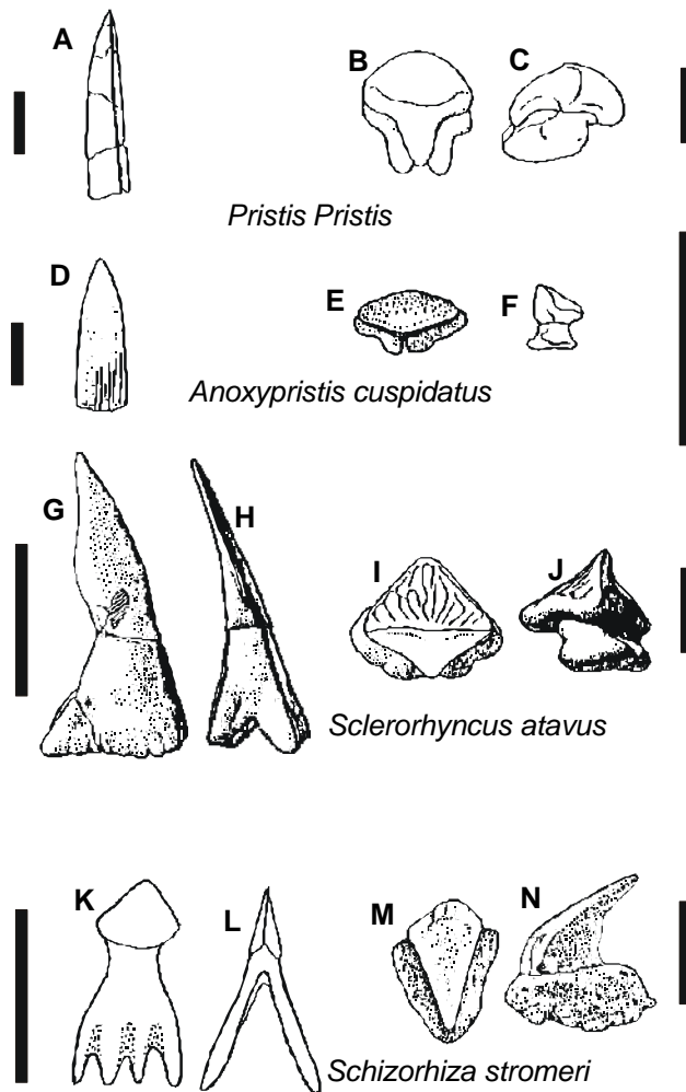
Figure 10. Rostral and oral teeth of sawfish. A-C Pristis pristis : A) rostral tooth in dorsal view, B) oral tooth in dorsal view, C) oral tooth in lateral view. D-F Anoxypristis cuspidatus : D) rostral tooth in dorsal view, E) oral tooth in dorsal view, F) oral tooth in lateral view. G-J Sclerorhynchus atavus : G) rostral tooth in dorsal view, H) rostral tooth in posterior view, I) oral tooth in dorsal view, J) oral tooth in lateral view. K-N Schizorhiza stromeri : K) rostral tooth in dorsal view, L) rostral tooth in posterior view, M) oral tooth in dorsal view, N) oral tooth in lateral view. Scale bars for rostral teeth = 1 cm. Scale bars for oral teeth = 1 mm.
