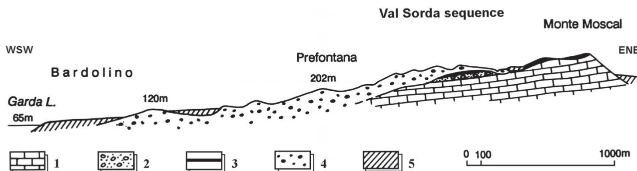
Figure 2. Geological section across the Garda moraines and Mt. Moscal. 1: bedrock; 2: till and fluvioglacial deposits (late middle Pleistocene); 3: loess (upper Pleistocene); 4: moraine ridges (late Pleistocene); 5: fluvial deposits (Holocene) (modified from Accorsi et al. , 1990).
