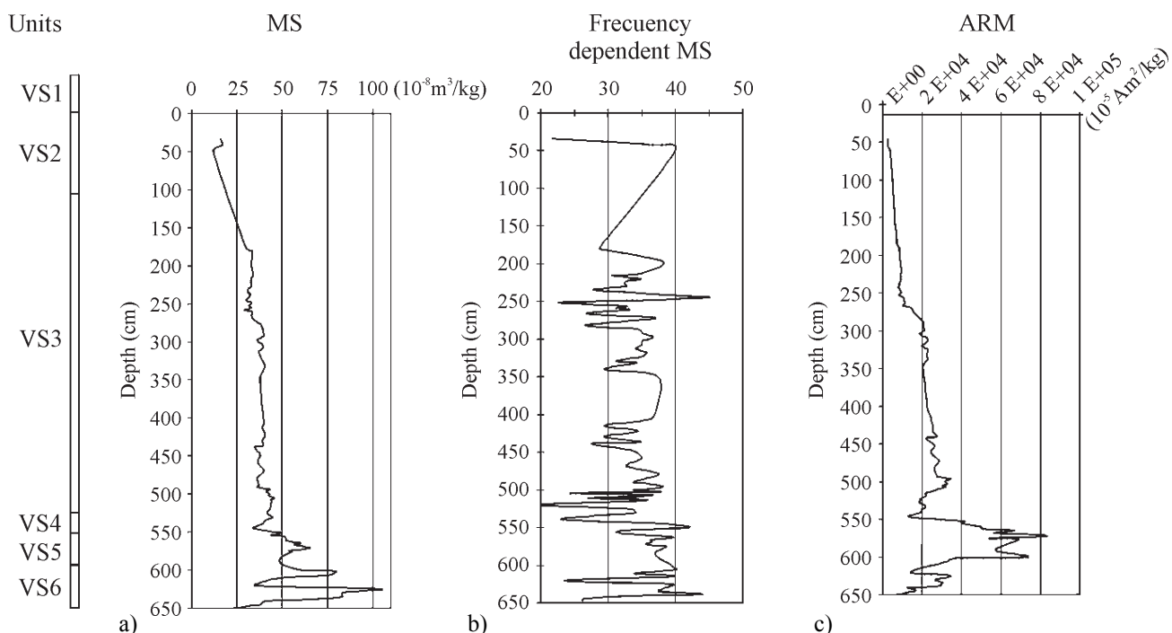
Figure 11. Magnetic susceptibility results from the Val Sorda profile. a) Mass specific magnetic susceptibility; b) frequency dependent susceptibility; and c) anhysteretic remanence magnetization.
