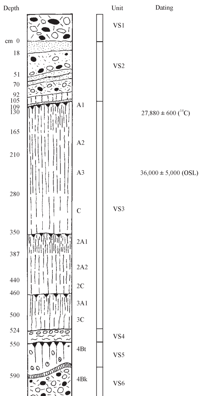
Figure 3. The stratigraphic sequence of the Val Sorda profile. Units and provided in former publications are indicated. Datings (in yr BP) from Cremaschi et al. (1987) and Accorsi et al. (1990); OSL: Optical Stimulated Luminescence.
