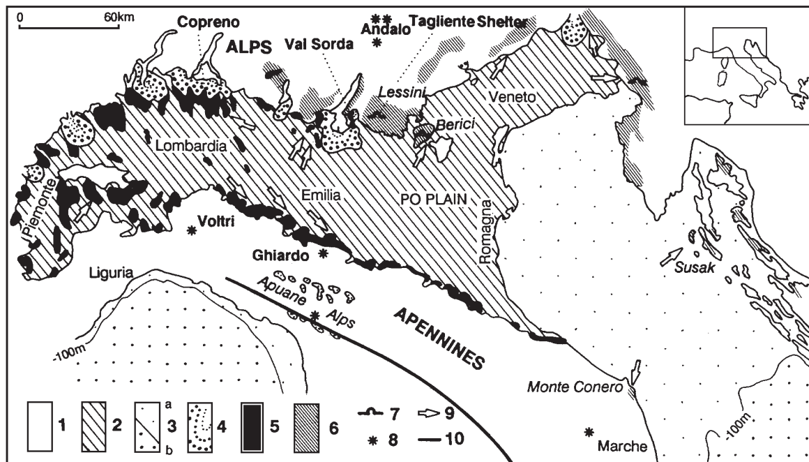
Figure 1. Loess distribution in northern Italy (modified from Cremaschi, 1990a). The geographic position of the Val Sorda profile is indicated. 1: Pre-Quaternary rocks; 2: Late Pleistocene and Holocene alluvial plain; 3: present day sea extent, a: less than 100 m deep, b: more than 100 m deep; 4: Pre-Alpine and Apennine moraine systems; 5: loess deposits on fluvial terraces, fluvio-glacial terraces, and moraine ridges; 6: loess deposits on karstic plateaus; 7: loess in caves or shelters; 8: loess on erosional surfaces; 9: direction of dominant winds during loess sedimentation; 10: possible southwest boundary of loess sedimentation during Late Pleistocene.
