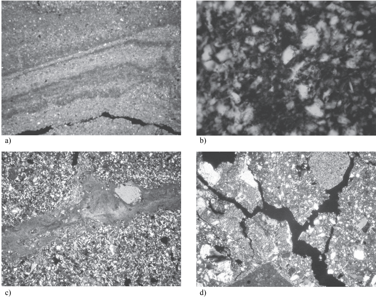
Figure 7. Micromorphological characteristics of some Val Sorda levels. a) Detail of sedimentary feature consisting of layers or lenses of very compact fine and light material, strongly \text{CaCO}_3 impregnated (1.6x XPL; VS2/105-109 cm); b) loess deposit in the Chernozem soil, rich in organic matter and containing iron impregnations (10x PPL; VS3/130-165 cm); c) iron-rich clay intercalation in the groundmass of the lower Chernozem soil (1.6x PPL; VS3/460-500 cm); d) subangular polyhedral aggregates of the Eemian paleosol (1.6x XPL; VS5/550-590 cm).
