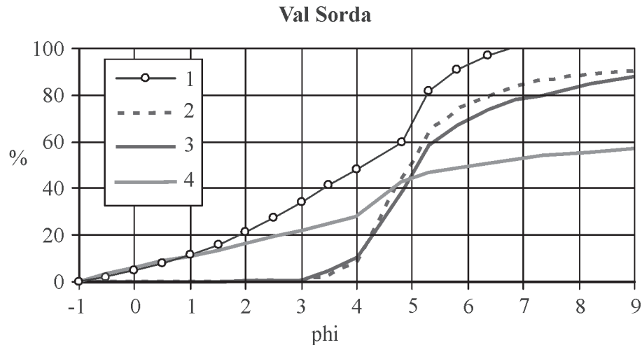
Figure 5. Some significant cumulative grain size curves from the Val Sorda profile. 1: Colluviated loess, where the sand and silt fractions are present in nearly equal amounts (VS2/51–60 cm); 2: loess curve; main component is silt (>80%), sand and clay are in low percentages (sand ~10%) (VS3/210–280 cm); 3: Chernozem paleosol formed in loess showing textural characteristics similar to curve 2 except for higher clay content (VS3/350–387 cm); 4: curve from an horizon of the rubefied paleosol formed in till; main component is clay (~47%), in consequence of strong pedogenetic activity; sand and silt (respectively ~28 and 25%) are also quite common (VS5/570–590 cm).
