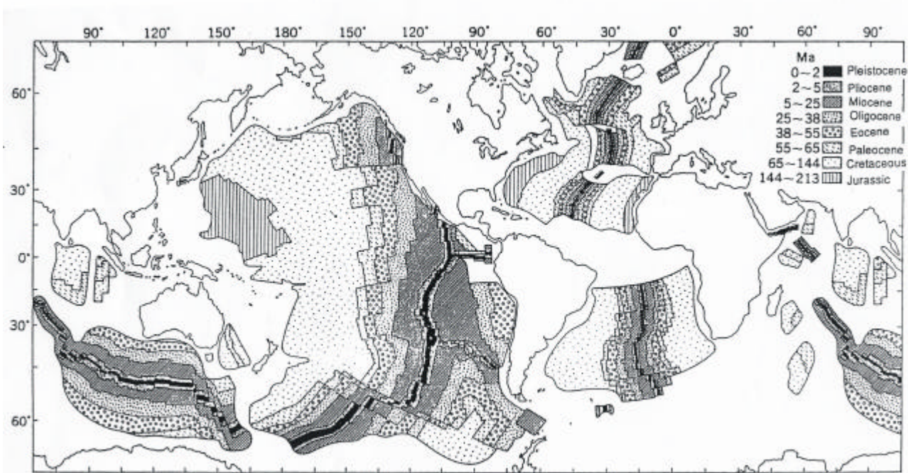
Figure 1. Isochron and age map of ocean basins and marginal basins (modified from Pitman et al. , 1974, and Tamaki and Honza, 1991).
