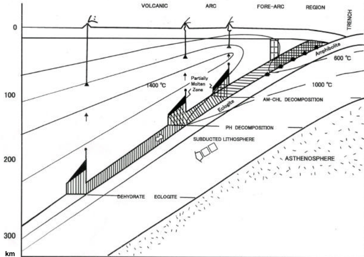
Figure 2. A plausible model for the migration of H_2O and the generation of basalt magmas in subduction zones. The hydrated slab are formed by addition of slab-derived H_2O (solid arrows) beneath the fore-arc region and should be dragged downward on the slab by the subduction of the oceanic plate. Amphibole (AM) and chlorite (CHL) in the dragged hydrated peridotite layer decompose to release H_2O at around 100 km just beneath a volcanic front, phlogopite (PH) decompose at around 150 km depth, and lawsonite-eclogite decomposes at around 250-300 km depth beneath the back-arc side of a volcanic arc. When the hydrated peridotite reaches the region with the solidus temperature of hydrous peridotite, partial melting takes place to produce initial magmas. Successive addition of H_2O to the region expands the partially molten zone upwards, and the degree of partial melting in this zone increases upwards. From the top of the partially molten zone a mantle diapir starts rising. The mantle diapirs must go through the region with temperatures higher than 1,400^\circ\text{C} and stop rising to release primary magmas. The depth of magma segregation from a mantle diapir is deeper in the back-arc side. It should be pointed out that the solidus temperature of hydrous peridotite cannot be attained in normal subduction zones. It follows that no magma can be produced by partial melting of the hydrous column beneath the fore-arc region (modified from Tatsumi, 1989).
