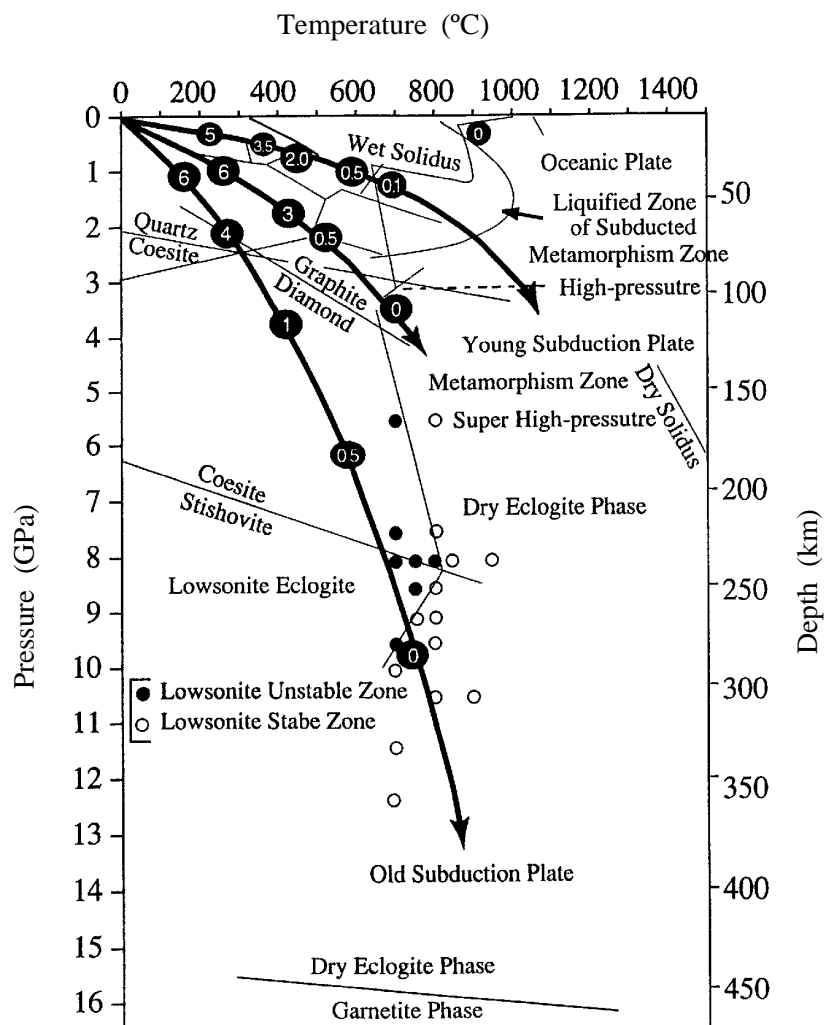
Figure 3. Mid-oceanic ridge basalt (MORB) - H 2 O phase diagram (modified from Okamoto et al. , 1997). Numbers in circles show the weight percent of H 2 O in the subducted slab. The downward dragged hydrous slabs can release H 2 O into the mantle, but young subducted slabs could not release H 2 O into the mantle, as they melt itself at shallow depth.
