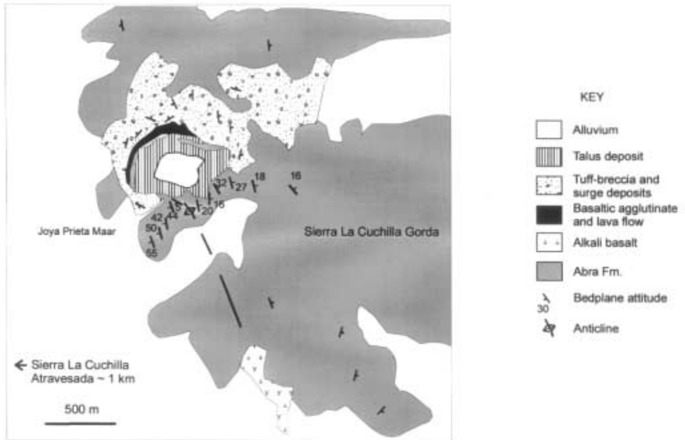
Figure 7. Simplified geologic map of the Joya Prieta maar and its surroundings. The location of this map is marked in Figure 2b.
