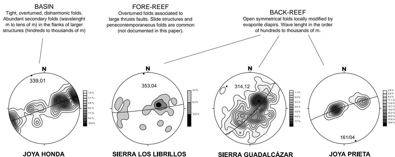
Figure 12. Summary of the results obtained in the structural analysis of data collected along the west-central margin of the VSLPP.
