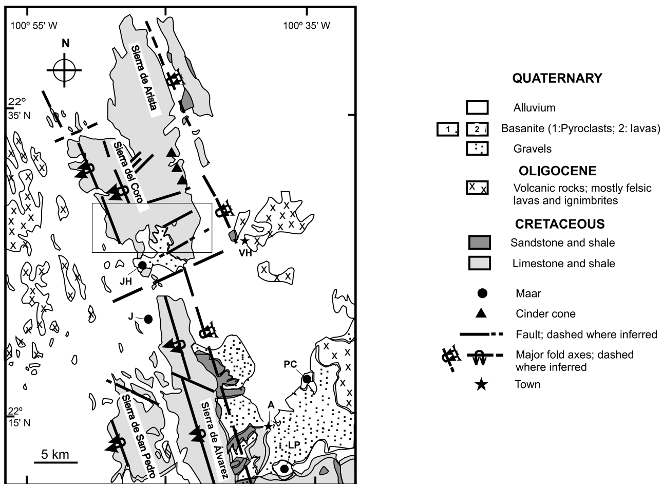
Figure 4. Generalized geologic map of the Sierra de Álvarez-El Coro anticlinorium. Box north of JH enclose the area where data was compiled for the structural analysis of Sierra del Coro. Towns: VH = Villa Hidalgo; A = Armadillo. Other maar volcanoes: J = Joyuela; LP = Laguna de los Palau; PC = Pozo del Carmen. Modified from Aranda-Gómez and Luhr (1996). The location of Figure 4 is marked on Figure 2b.
