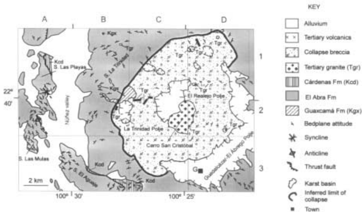
Figure 10. Generalized geologic map of Sierra de Guadalcázar (SG). Note the presence of large karstic basins at the collapse area. It is likely that the Guadalcázar-El Ábrigo Polje, together with the northern and northwestern limit of the collapse breccia, roughly delineates the area disturbed by the tectonically thickened anhydrite; the most perturbed area is around the outcrops of the Guaxcamá Formation. Modified from Torres-Hernández (1994). G-Guadalcázar.
