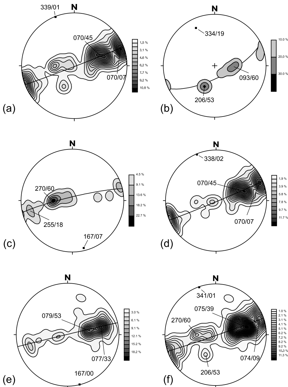
Figure 6. Contoured plots of poles to bedding projected into the lower hemisphere of an equal area net. (a) Data collected along the southern rim of the Joya Honda maar ( n=130 ), (b) and (c) detailed measurements in second order folds exposed in the southern rim of the maar ( n=10 and n=22 , respectively), (d) Same as plot (a) after filtering out the data corresponding to obvious second order folds [i.e., (b) and (c)], (e) compiled structural data ( n=66 ) shown in the regional map (see box in Figure 1c for location) of the southern part of Sierra El Coro (Aranda-Gómez and Labarthe-Hernández, 1977), and (f) combined data set ( n=196 ) using the information of both the southern part of Sierra El Coro and Joya Honda. All the diagrams show the great circle fitting best to the girdle and its pole (p axis).
