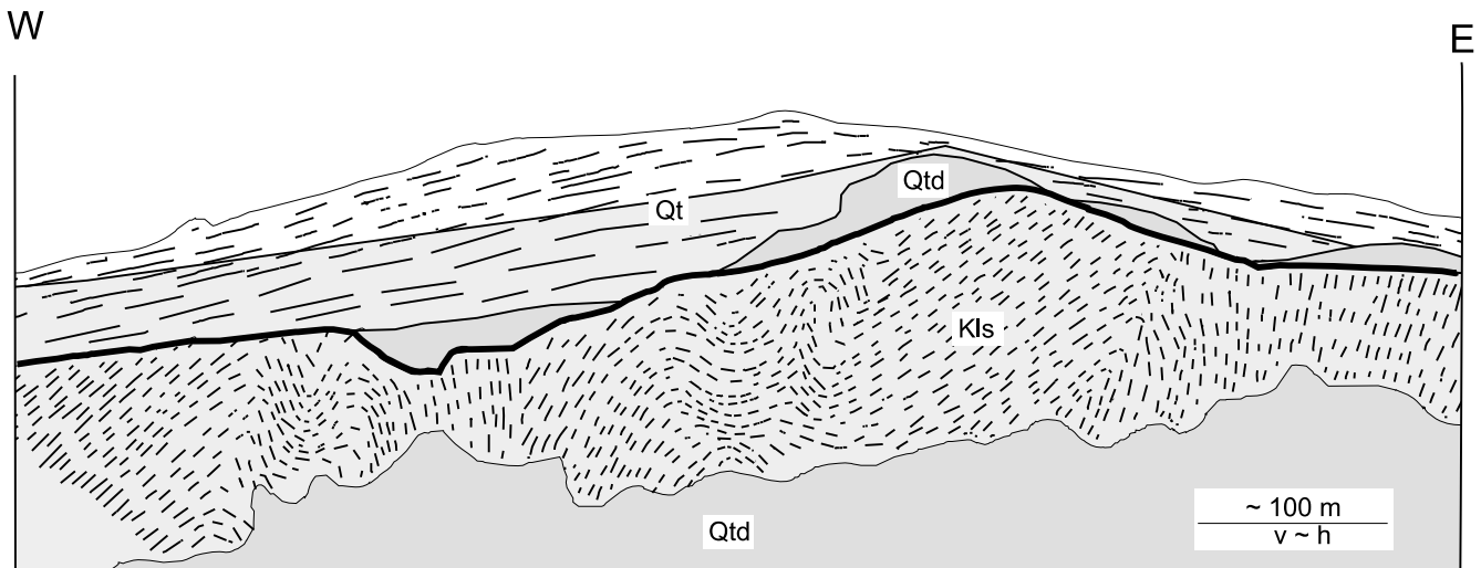
Figure 5. Geologic sketch of the northern wall of Joya Honda. The diagram was prepared tracing the contacts between the different lithologic units and the bedding in the marine sediments and pyroclastic sequence on a series of panoramic photos. The maximum height of the crater's wall is ~300 m. Note that the overall shape of the structure in the limestones (Kls) is that of a slightly overturned anticline. However, in the southwestern limb of the structure there are several second-order folds. Common types of second-order folds observed on the walls of the crater and around the maar are chevron-, box- and cusped-type folds. The Quaternary tephra (Qt) forms a broad open pseudofold for the reason of the presence of drape bedding due to the irregular surface (heavy line) in which was accumulated. Qtd = Talus deposit (simplified from Aranda-Gómez et al., 1993).
