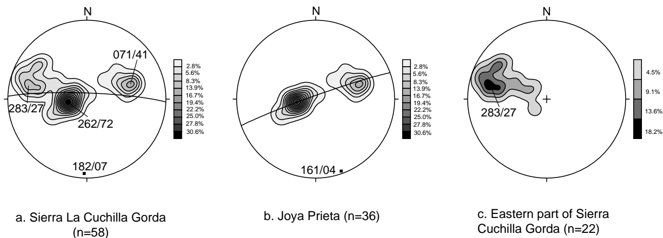
Figure 8. Contoured plots of poles to bedding projected into the lower hemisphere of an equal area net. (a) data collected in Sierra La Cuchilla Gorda traverse (n=58). (b) data collected in the southern rim of the Joya Prieta maar (n=36). (c) Cuchilla Gorda set (n=22) after filtering out the data corresponding to the anticline exposed in the southern wall of Joya Prieta. Beds in the eastern portion of the fold were disrupted and rotated by a cataclastic fault zone oriented N5°E/60°SE.
