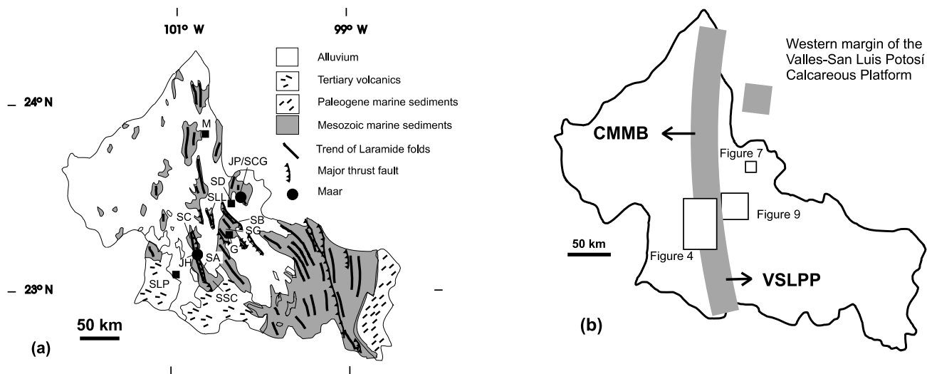
Figure 2. (a) Geologic sketch map of the State of San Luis Potosí. It shows the regional trend of Laramide structures, major known thrust faults (after de Cserna, 1992, and Torres-Hernández and Tristán-González, 1994), and the location of sierras de Álvarez (SA), El Coro (SC), Santa Catarina (SSC), Los Librillos (SLL), Guadalcázar (SG), La Cuchilla Gorda (SCG), and Buenavista. Quaternary maars are Joya Honda (JH) and Joya Prieta (JP), and towns mentioned in the text are Santo Domingo (SD), Guadalcázar (G), San Luis Potosí city (SLP), Matehuala city (M). (b) Approximate location of the transitional zone between the CMMB and VSLPP.
