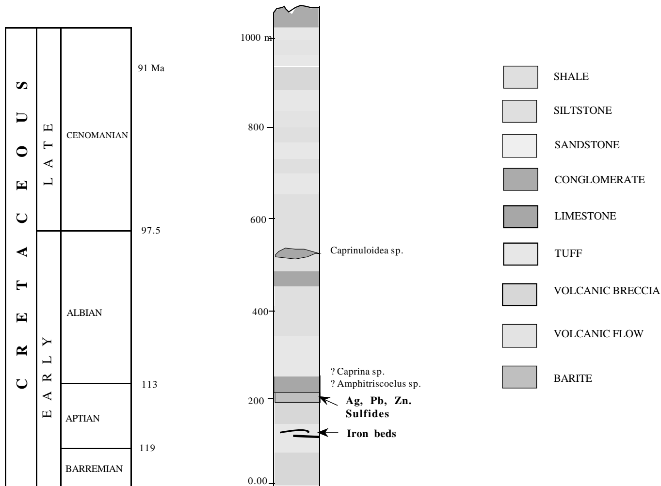
Figure 4. Stratigraphic column of the La Minita-La Hueca area.
