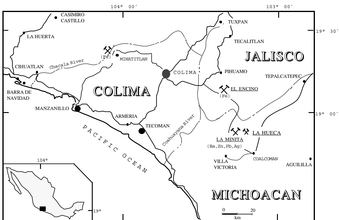
Figure 1. Location map of the La Hueca deposit area.
