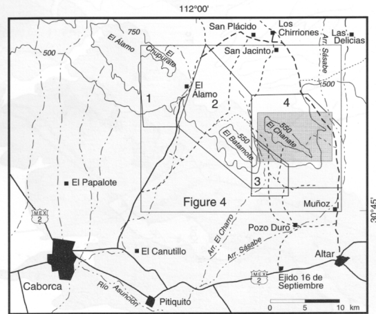
Figure 3. Location of the Sierras El Chanate, El Batamote and Puerto El Álamo. Large inset indicates location of Figure 4. Shaded inset indicates location of Figure 5. Sources of information for geologic map (Figure 4) are: (1) Willard, 1988; (2) Harrar, 1989; (3) McComb, 1987; (4) Jacques-Ayala, 1993.
