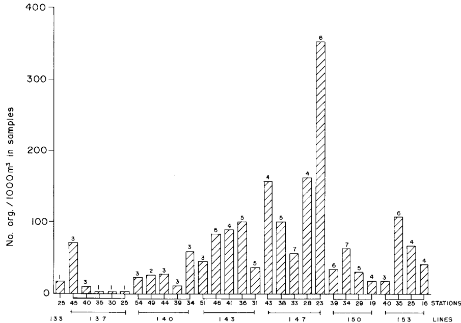
Fig. 6. Distribution of the estimated abundance of holoplanktonic polychaetes in the southwest region of Baja California, Mexico. Volume of water strained is estimated at 500-600 m 3 . Numbers above each column represent the richness of species.
